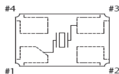
Land Pattern(REFERENCE)
