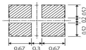
Land Pattern(REFERENCE)
